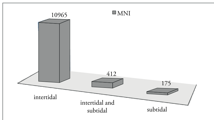
FIG. 9. Distribution (by MNI) of marine species according to viable bathymetric levels.
