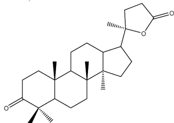
4 25,26,27-trisnor-20S-hidroxi-3-oxodammaran-24-oico-20,24-lactona
