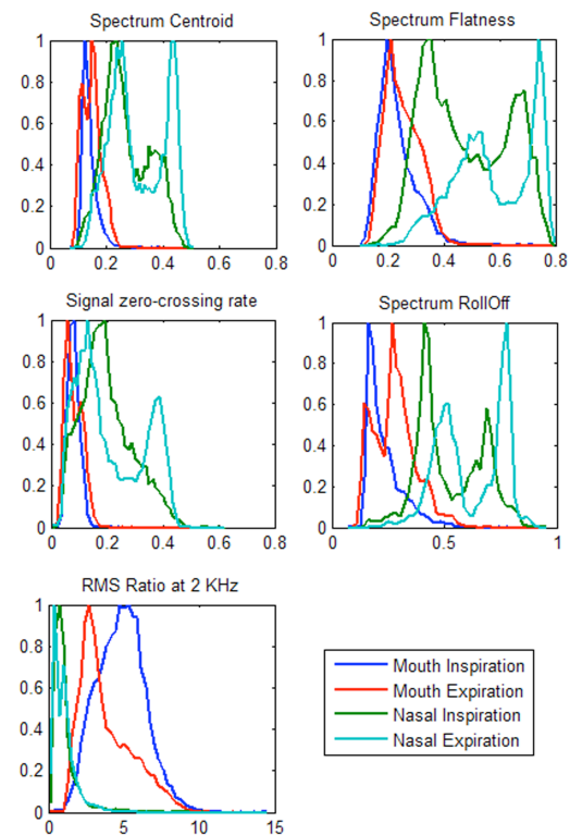
Fig. 3. Plot of extracted acoustic features (except MFCC) showing normalized distributions from the 4 respiratory
