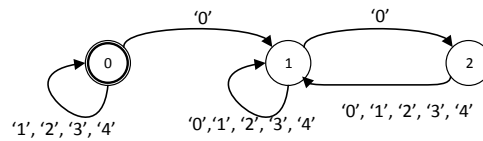
Fig. 2. State machine for respiratory movement identification
